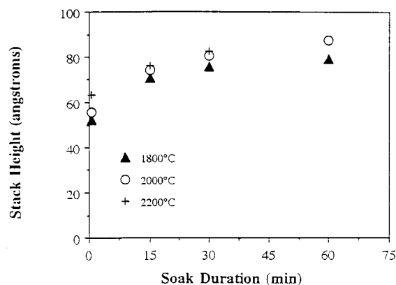
Figure 9 Influence of soak duration on stack height.
