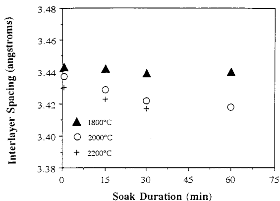
Figure 8 Influence of soak duration on interlayer spacing.
