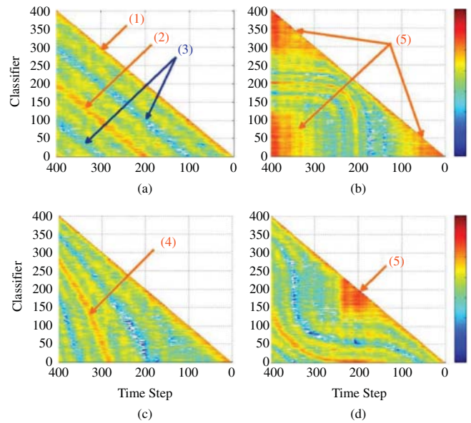
Fig. 8. Weight distribution (max in red, min in blue) over time for checkerboard dataset with (a) constant, (b) pulsing, (c) exponential, and (d) sinusoidal drift rate.
