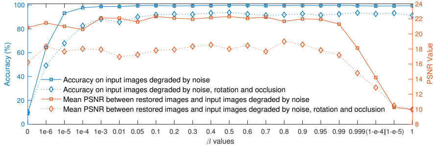
Fig. 6 Validation with different values of \beta using the Joint-Cap-Net on images degraded only by noise, and images degraded by combining effects from noise, rotation and occlusion.
