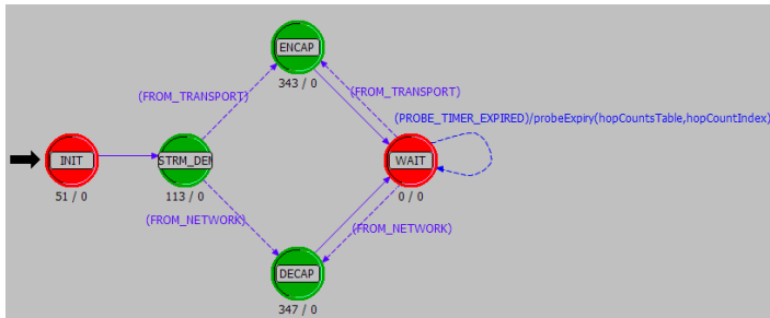
Figure 1: Updated ip_encap_v4 process model
