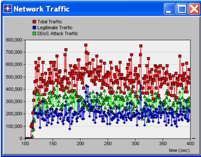
Figure 3: Direct UDP Flood Attack Traffic Distribution
