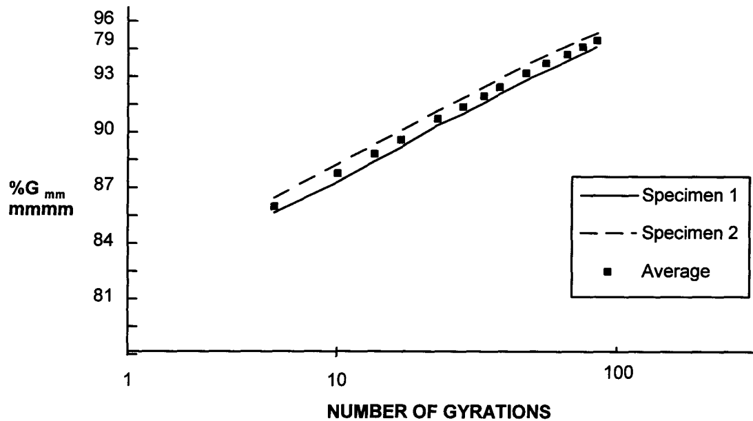
IH-43, 19.0 mm Nominal, 4.4% AC, Trial Blend 1
