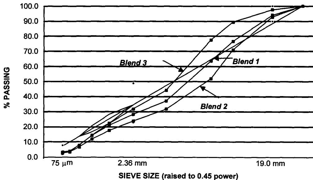
IH-43 Trial Gradations 19.0 mm Nominal Mixture
