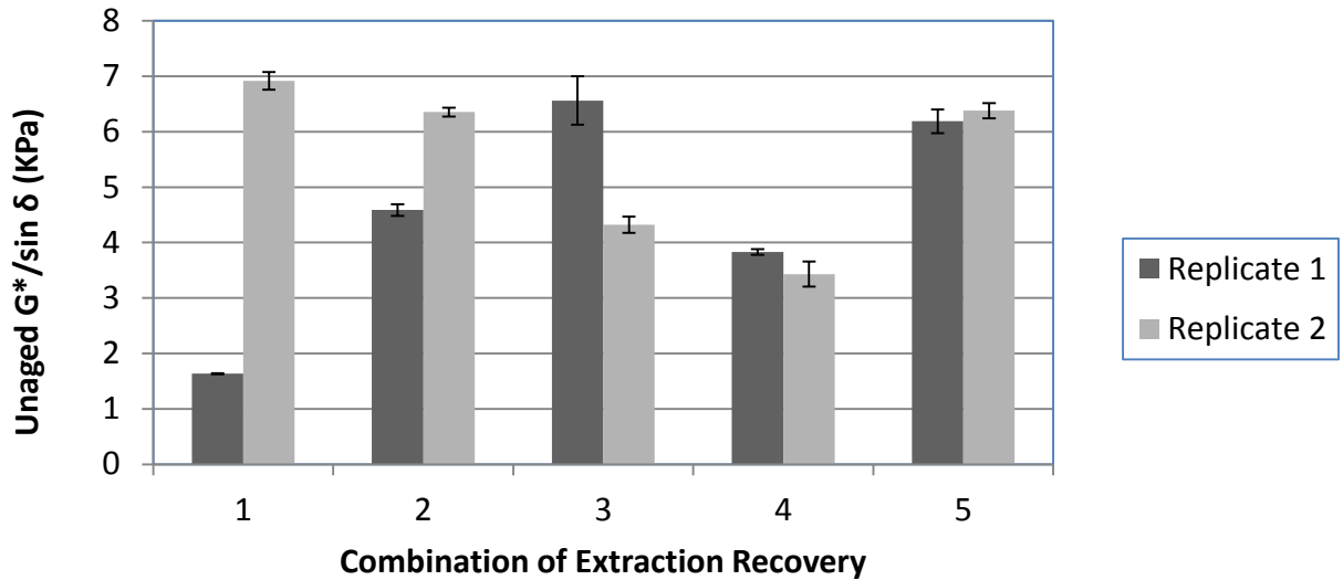
Figure 7-6. Comparison of Un-aged G^*/\sin \delta for Different Combination of Extraction and Recovery Procedure.
