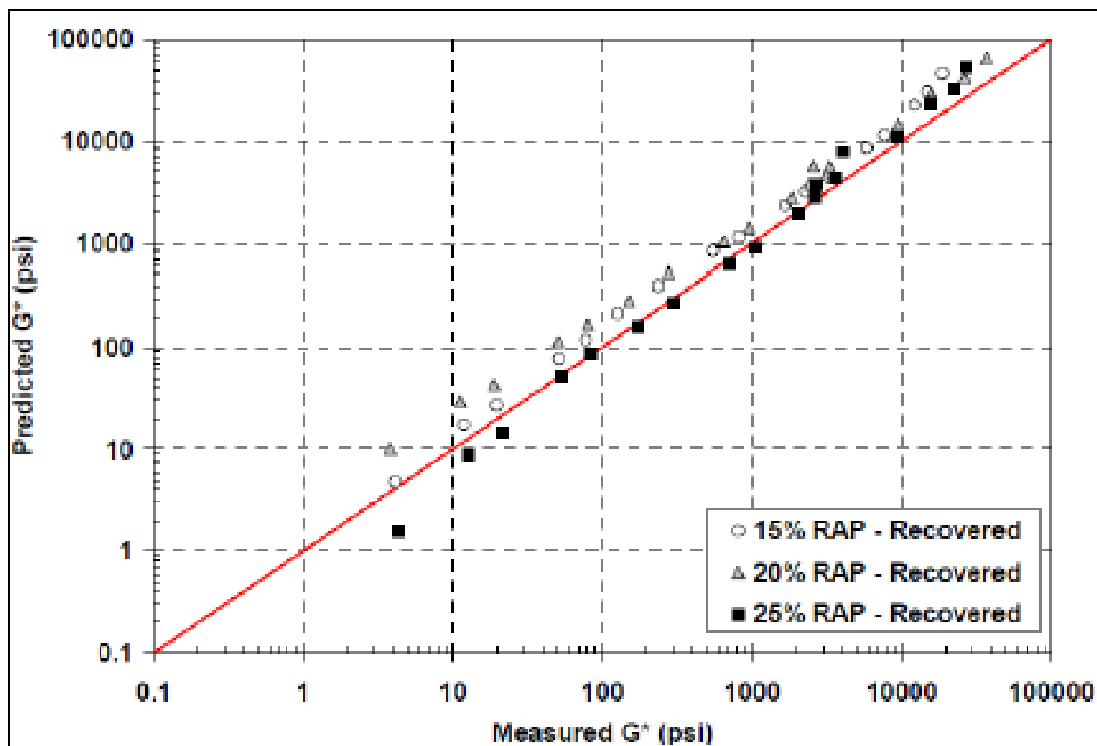
Figure 2-13. Evaluation of Degree of Blending Between RAP and Virgin Binder (74)
