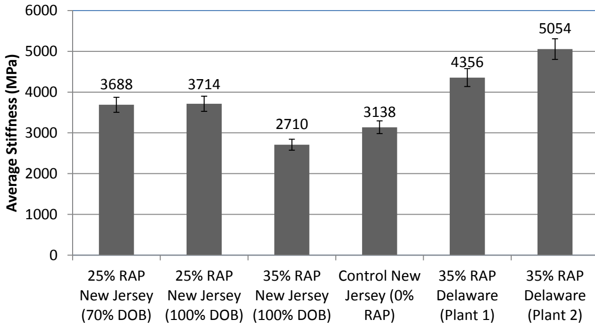
Figure 8-3. Stiffness Values for All RAP Mixtures
