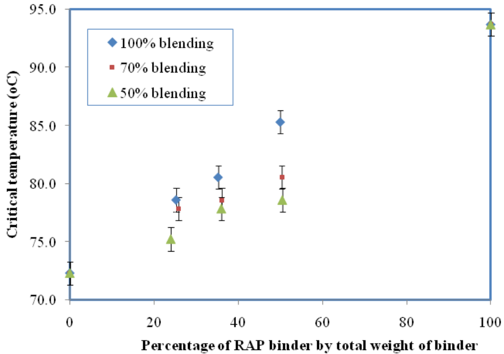
Figure 6-2. Blending Chart for PG 70-28
