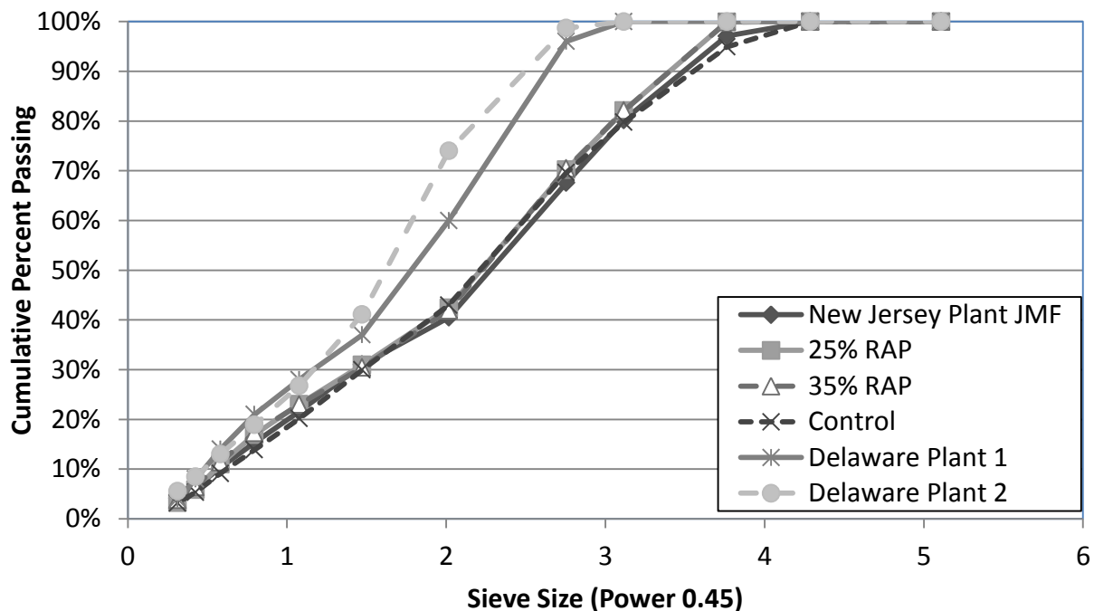
Figure 8-1 Plant and Laboratory Gradations Used in Study
