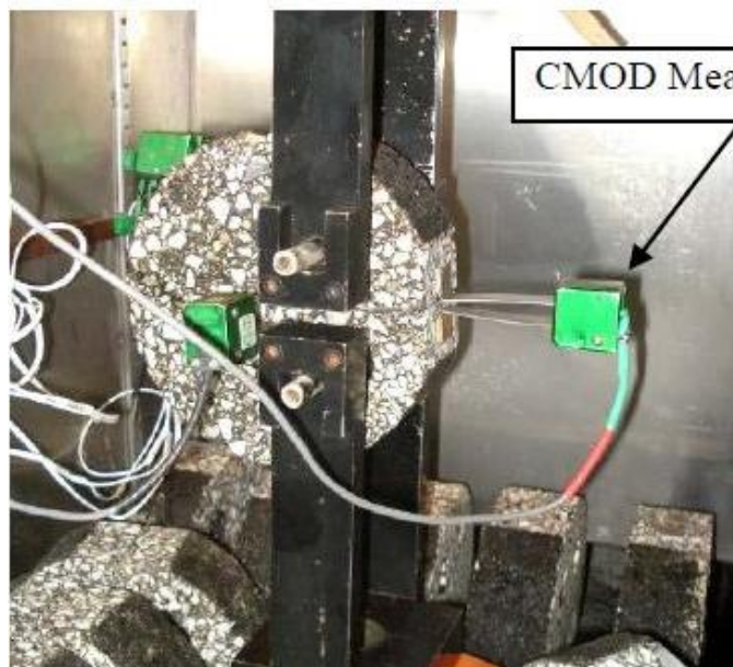
Figure 3-2. DCT Test Set Up
