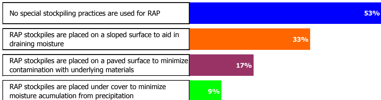
Figure 2-2. Summary of RAP Stockpiling Practices (9)
