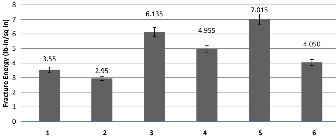
Figure 8-2. Fracture Energy for All RAP Mixtures
