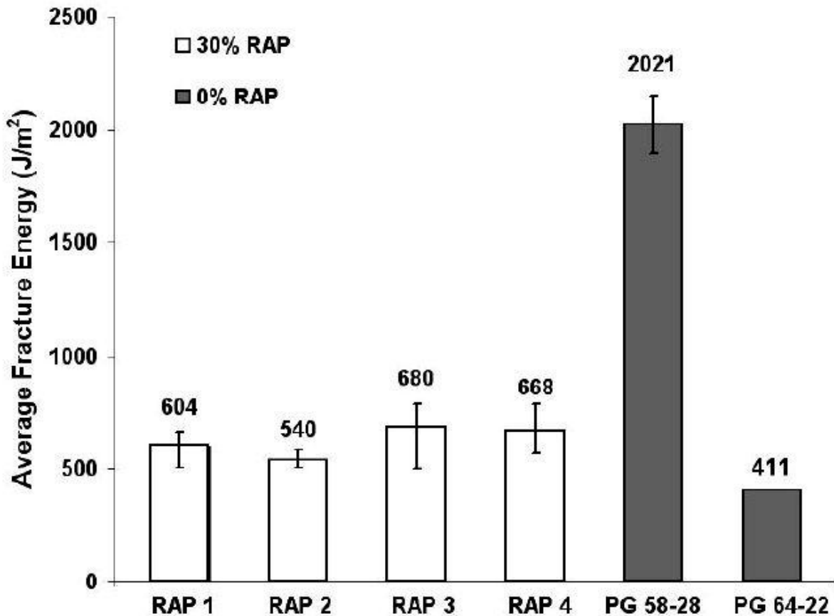
Figure 2-11. Average Fracture Energy for Zero Percent RAP and 30 Percent RAP Mixture. (66)
