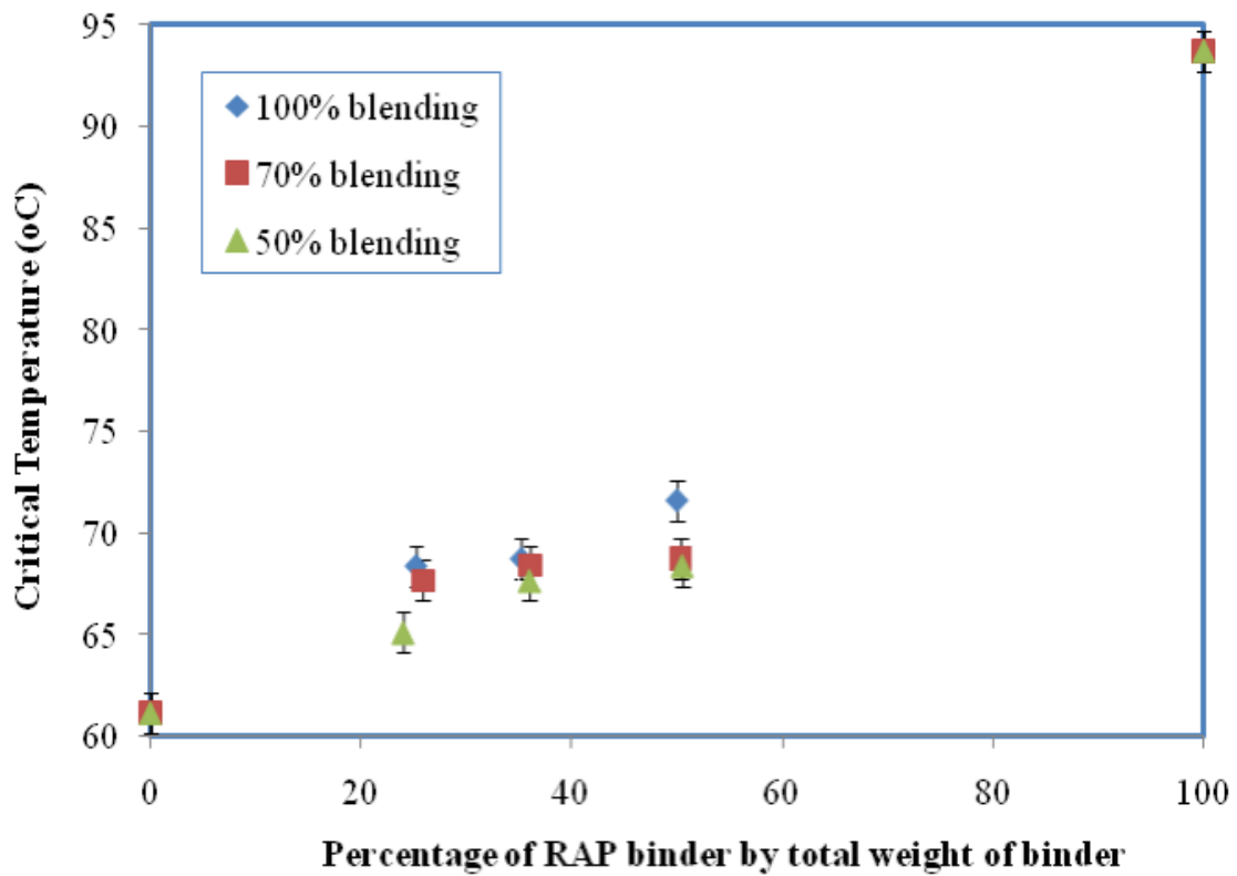
Figure 6-3. Blending Chart for PG 58-28
