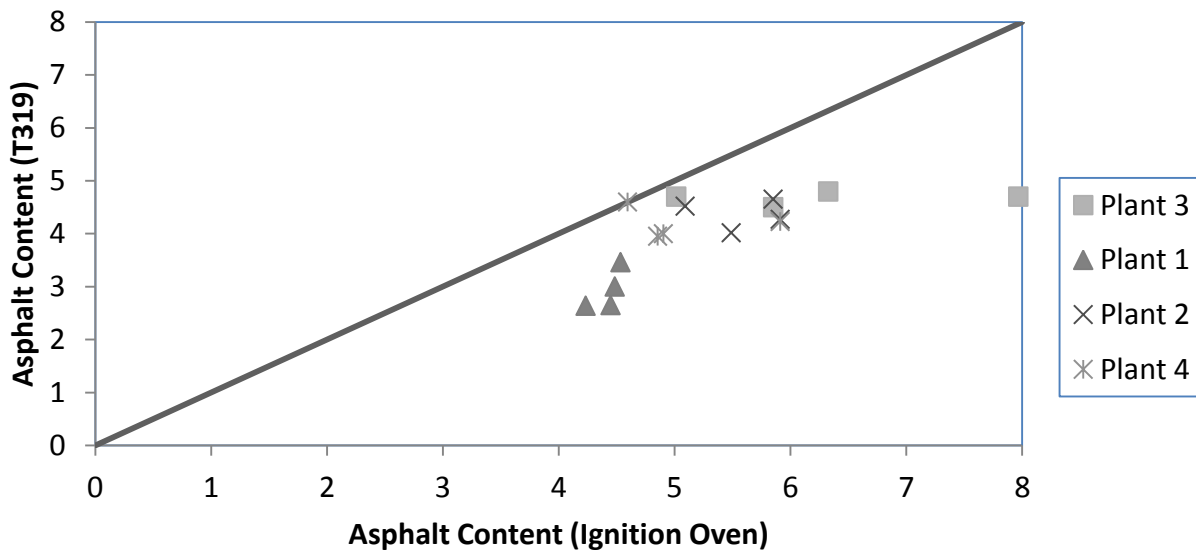
Figure 7-3. Comparison of AC for Ignition Oven and Extraction and Recovery (10)
