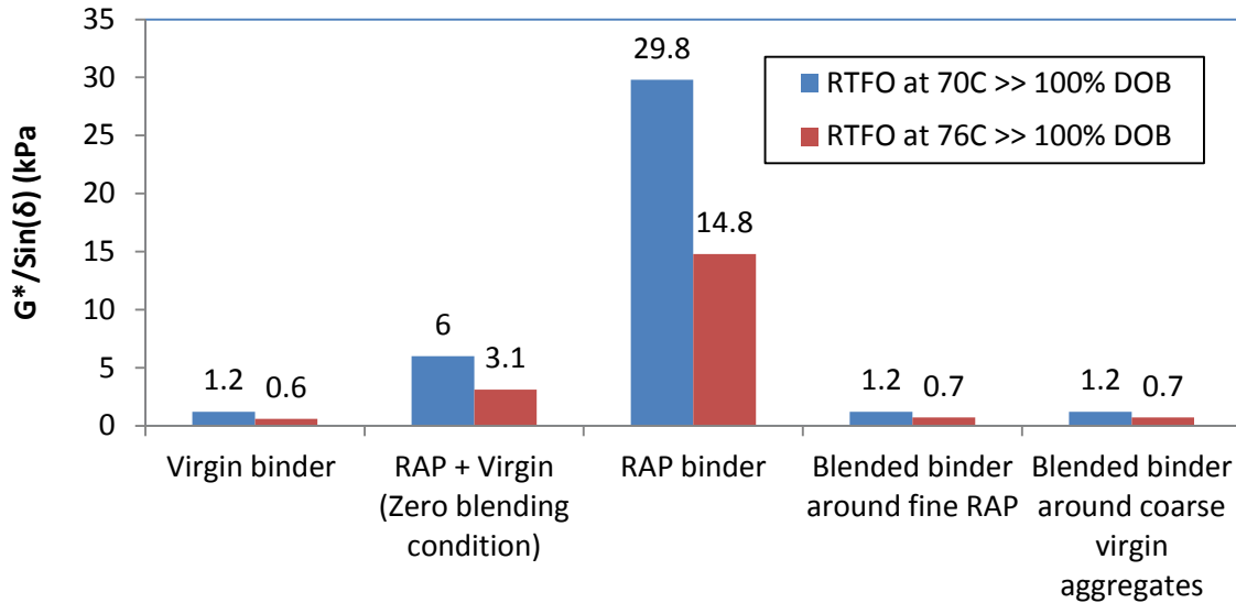
Figure 5-4. Comparison of RTFO G^*/\text{Sin}(\delta) at 76 °C and 70°C for Batch 2 of 35 Percent RAP.
