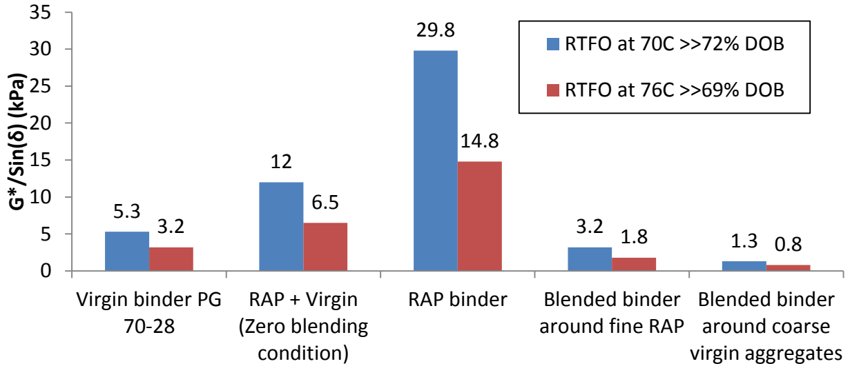
Figure 5-2. Comparison of RTFO G^*/\sin(\delta) at 76°C and 70°C For 25 Percent RAP.
