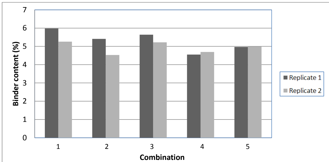
Figure 7-5. Binder Content of RAP for Different Combination of Extraction and Recovery Procedure.
