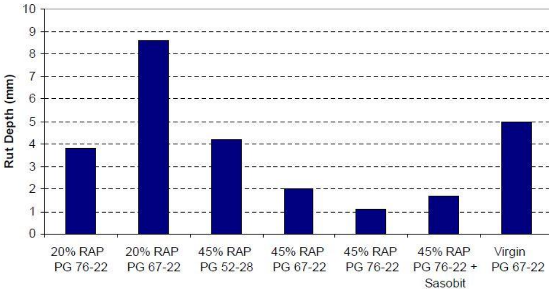
Figure 2-8. Field Rut Depths at 9.4 Million ESALs for the RAP Experimental Sections (9)
