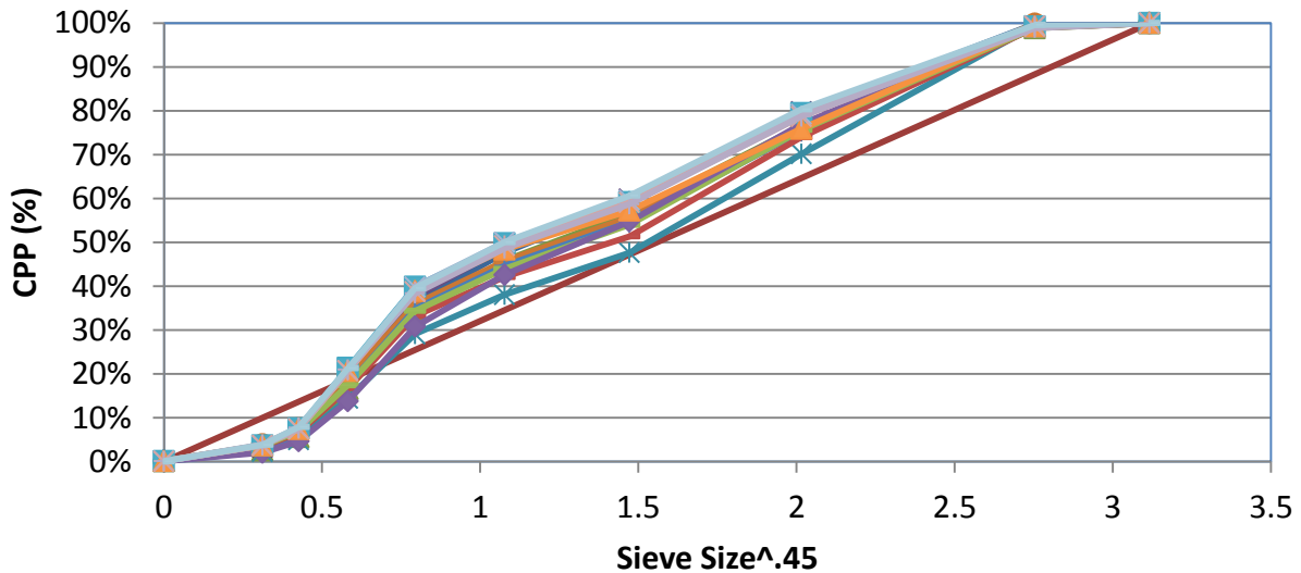
Figure 11-2 Plant B RAP gradations plotted against maximum density line
