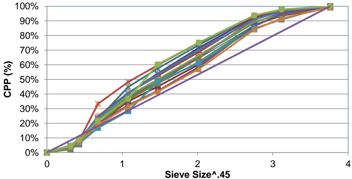
Figure 11-1. Plant A gradations plotted against maximum density line
