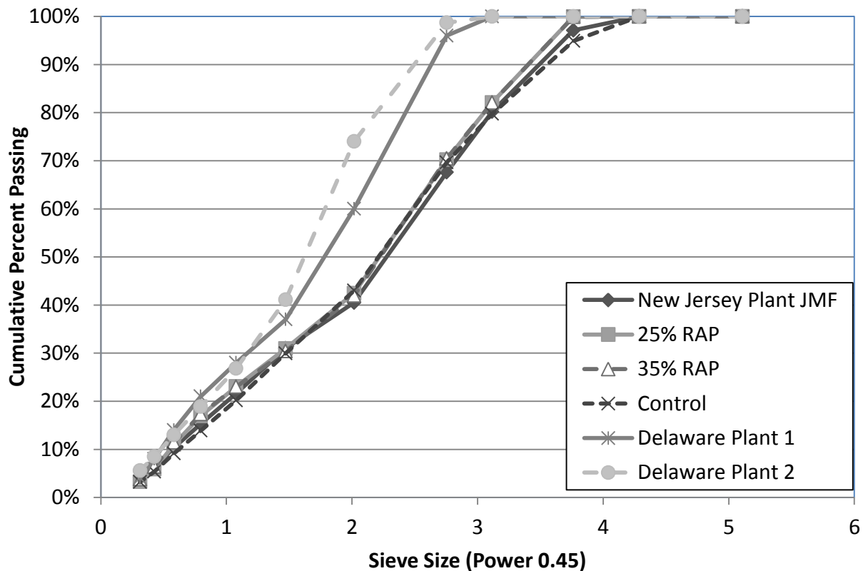
Figure 3-1 Plant and Laboratory Gradations Used in Study
