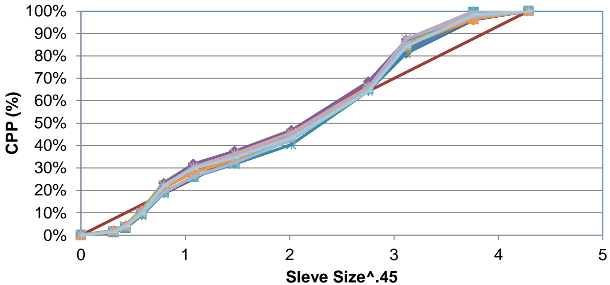
Figure 11-3. Plant C RAP gradations plotted against maximum density line
