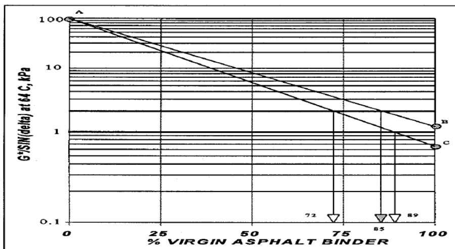
Figure 2-4. Specific Grade Blending Chart (48)
