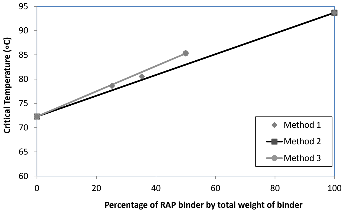
Figure 6-4. Blending Chart for PG 70-28 for 100 Percent DOB
