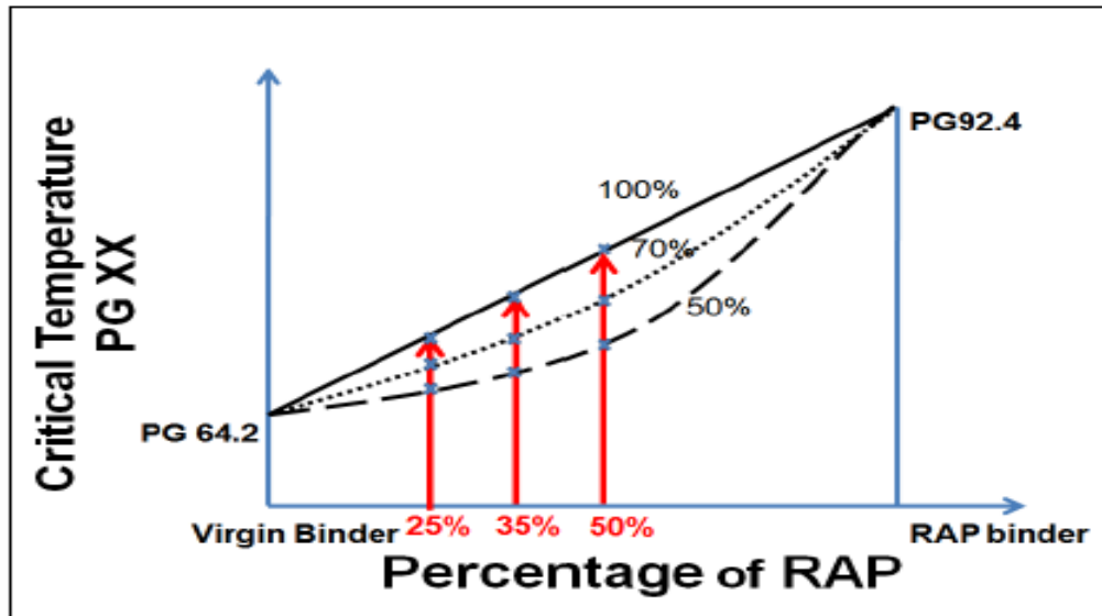
Figure 3-5. Graph Illustrating Details of Replicates Required to Develop Blending Chart for Different Degree of Blending
