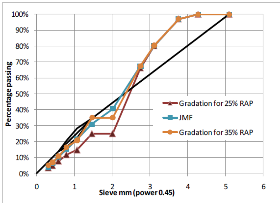
Figure 4-1. Gradation of the JMF and the Gap Gradation for 25 Percent and 35 Percent RAP
