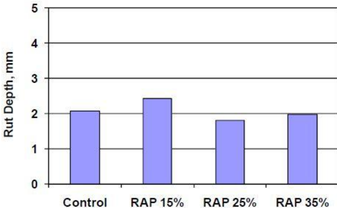
Figure 2-9. Rut Depth From APA Test (61)
