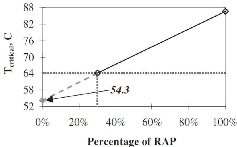
Figure 2-5. High-Temperature Blending Chart for Known RAP Percentage (49)
