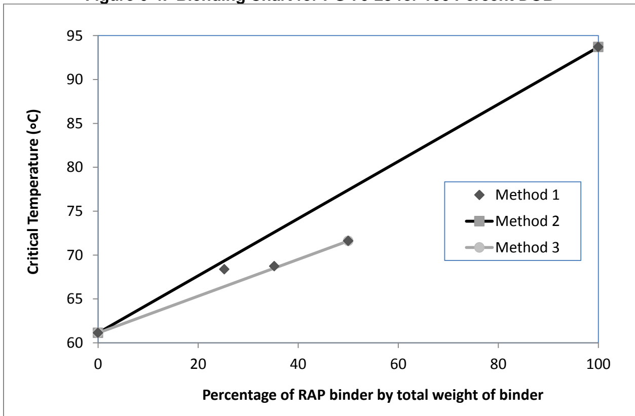
Figure 6-5. Blending Chart for PG 58-28 for 100 Percent DOB
