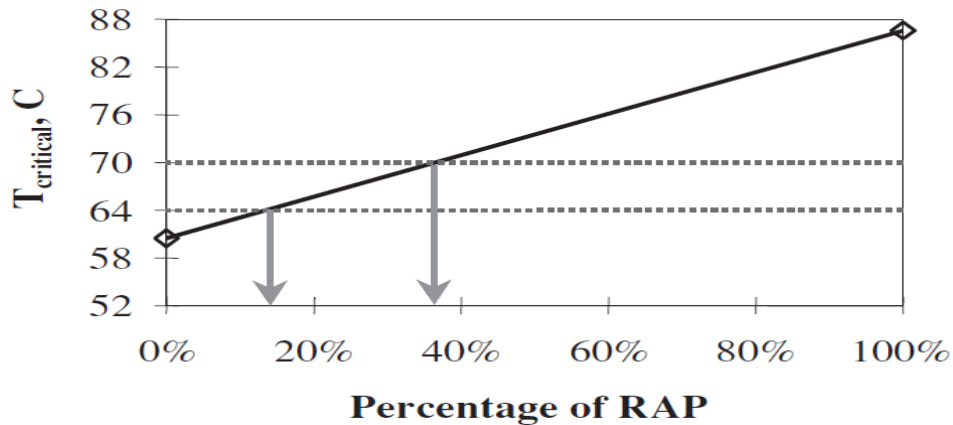
Figure 2-6. High Temperature Blending Chart for Unknown RAP Percentage (49)
