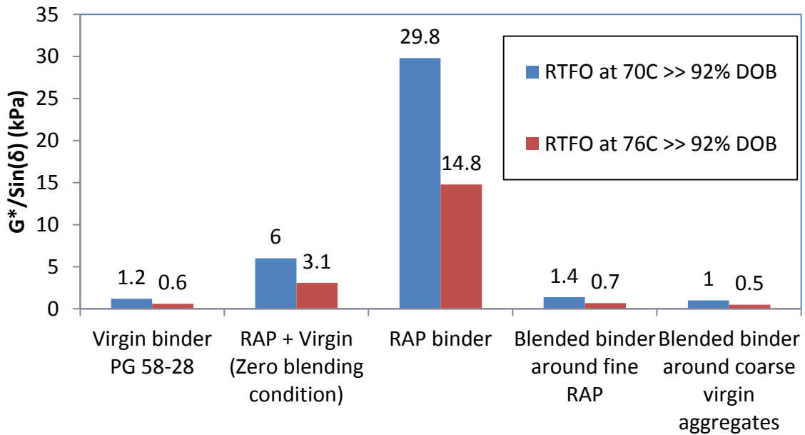
Figure 5-3. Comparison of RTFO G^*/\sin(\delta) at 76°C and 70°C For Batch 1 of 35 Percent RAP.
