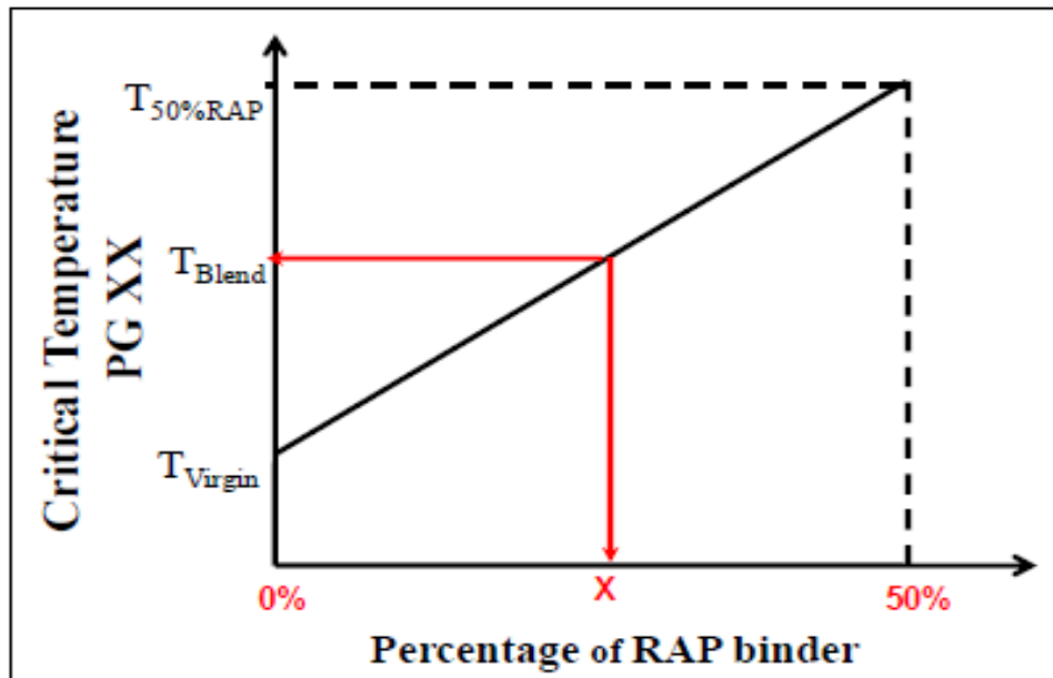
Figure 6-1. Method 3 Blending Chart to Determine Critical Temperature for Intermediate Percentage of RAP by Interpolating Virgin and 50 Percent RAP Binder
