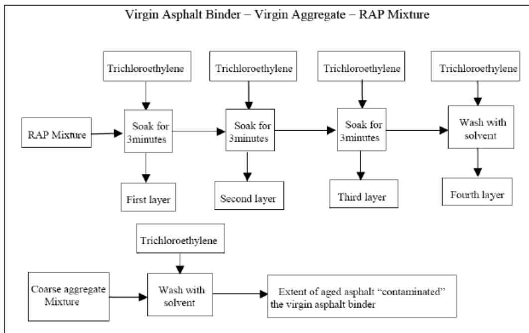
Figure 2-12. Staged Extraction-Recovery (57)
