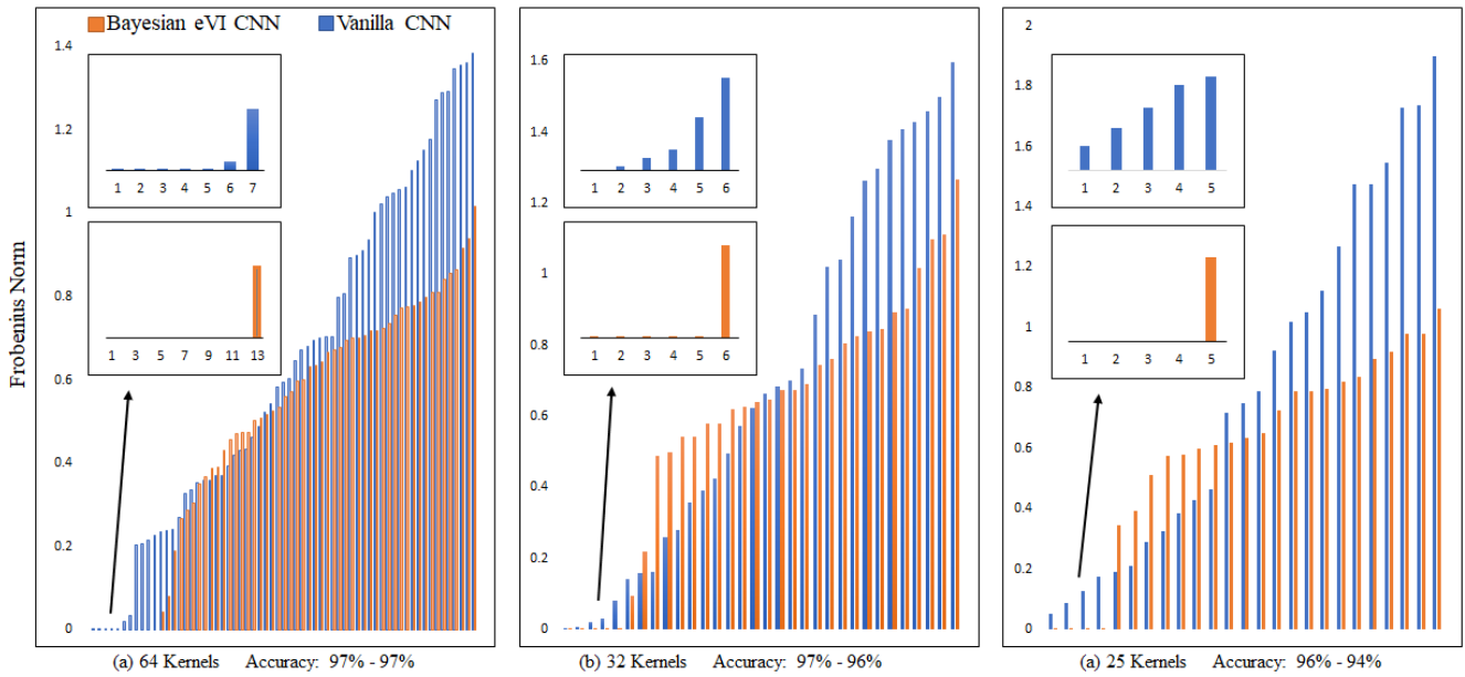
Fig. 3. The Frobenius norms of convolutional kernels for the Bayesian eVI and Vanilla CNNs with N = 64, 32, and, 25 for the MNIST dataset are presented. The zoomed sub-figures show kernels with small Frobenius norms. In all cases, Bayesian eVI CNN can discover zero kernels ( \|\cdot\|_F \leq 10^{-7} ). We consider that a Bayesian eVI CNNs provide a principled way to identify and iteratively remove zero kernels, i.e., self-compression.
