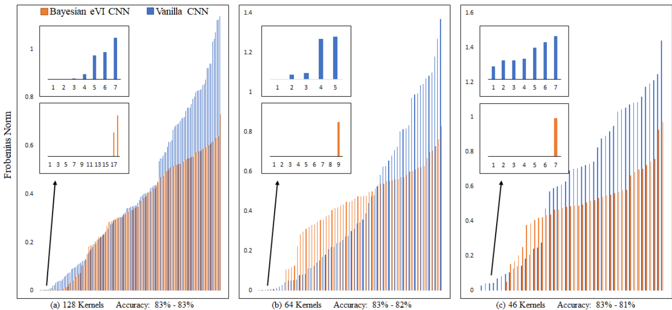
Fig. 4. The Frobenius norms of convolutional kernels for Bayesian eVI and Vanilla CNNs with N = 128, 64, and, 46 for the F-MNIST dataset are presented. The zoomed sub-figures show kernels with small Frobenius norm values. We note that for all cases, Bayesian eVI CNN can discover zero kernels and leads to self-compression.
