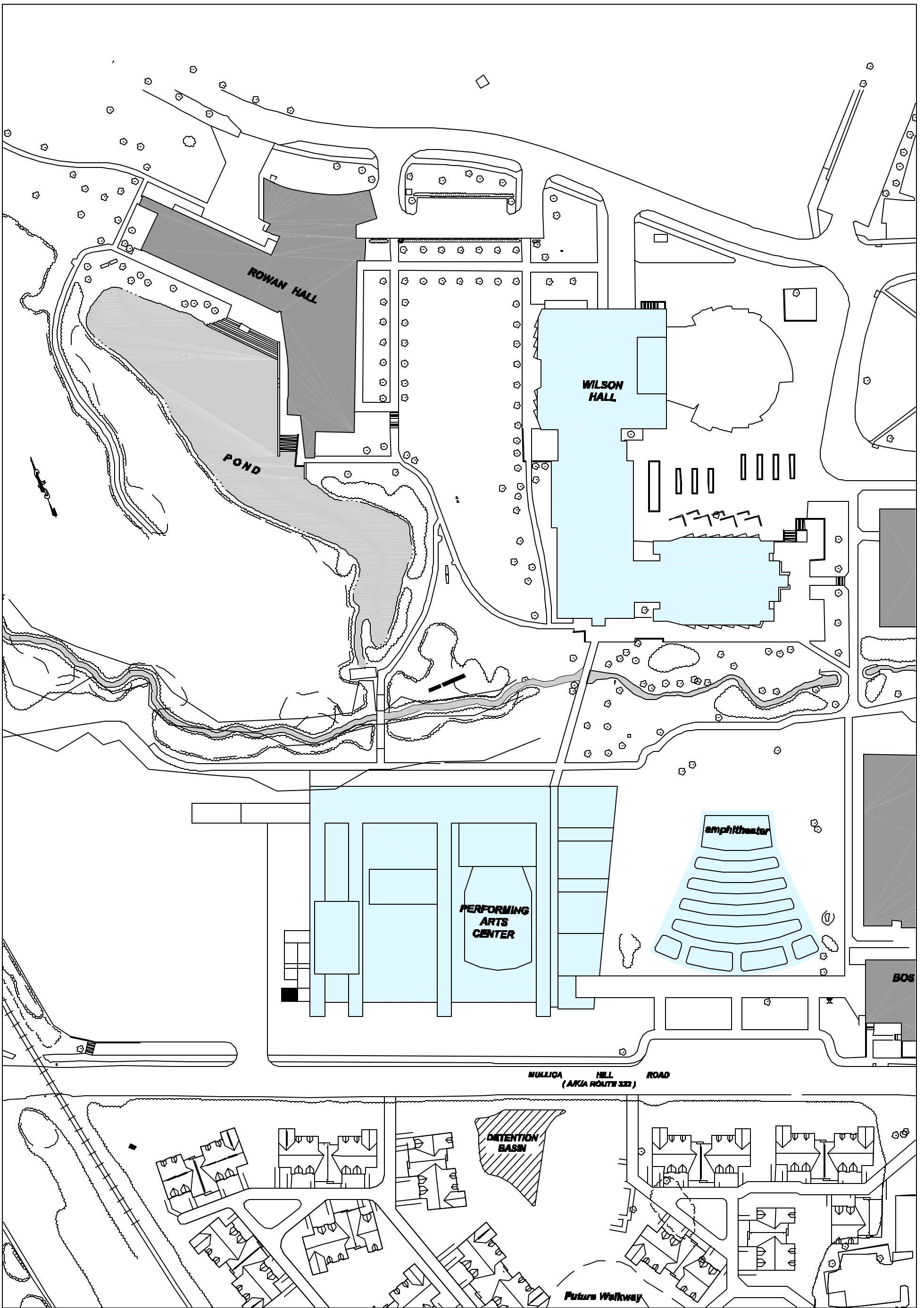
SITE PLAN - PHASE 2 SCALE: 1/100" = 1'-0"
