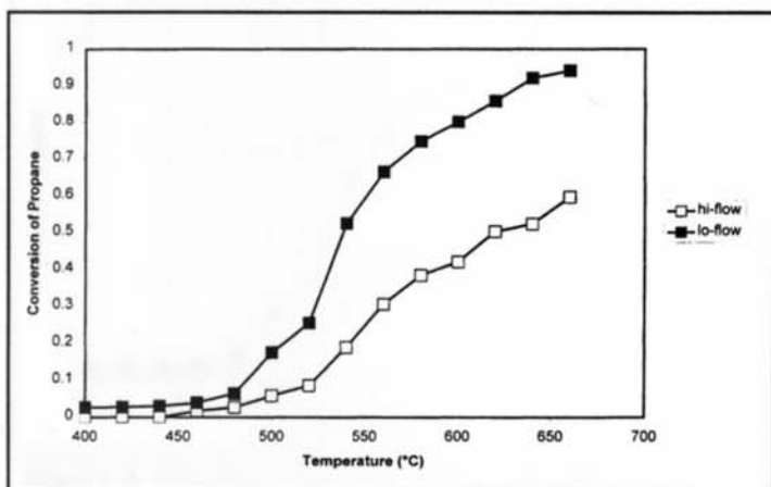
Figure 4. Results of light-off determination experiment.
