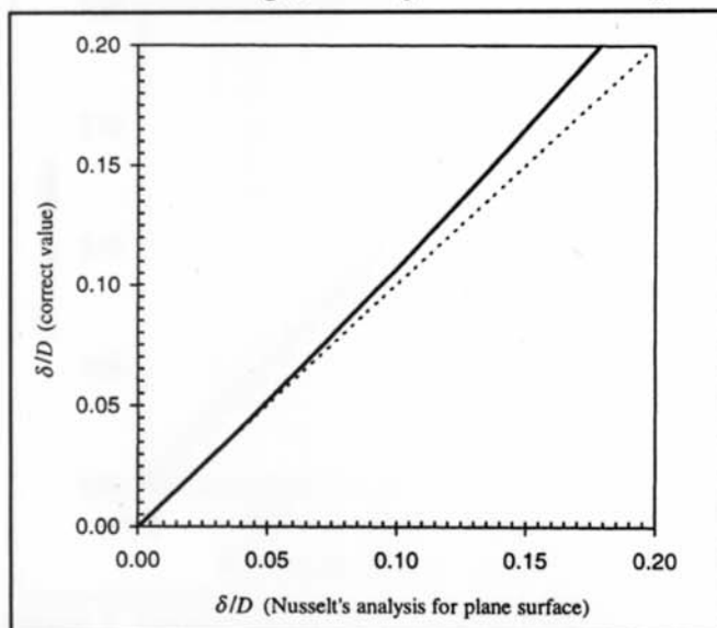
Figure 1- Correct versus approximate film thickness.
