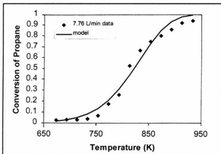
Figure 5. Comparison of model with experimental light-off curve data.
