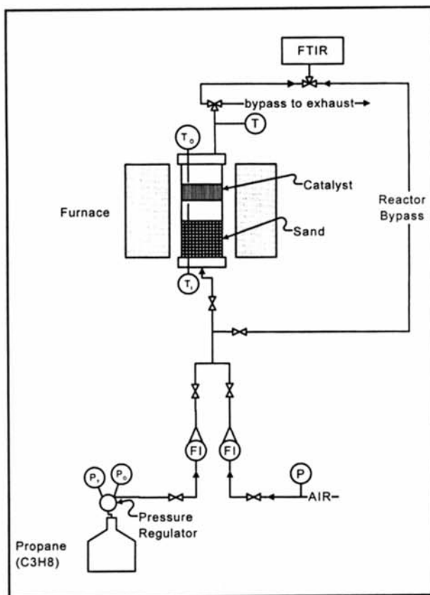
Figure 1. Experimental catalytic reactor.
