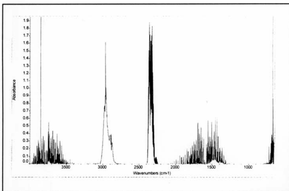
Figure 3. FTIR spectrum from the reactor outlet stream using an inlet concentration of 1000 ppm propane in air at a furnace temperature of 500°C.
