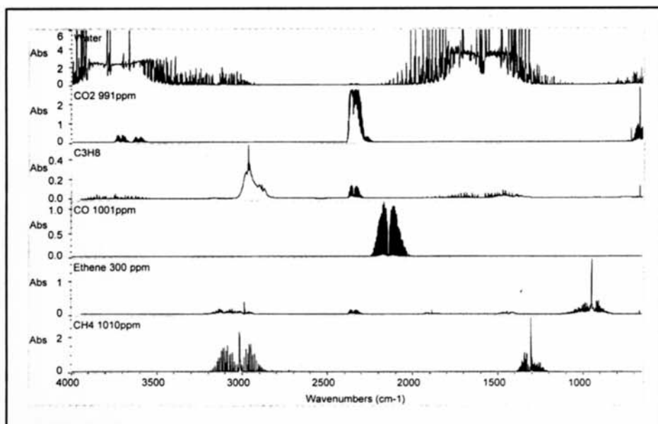
Figure 2. Standard spectra of possible absorbing compounds from reactor outlet.
