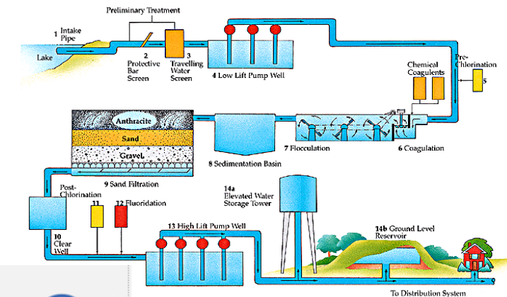
WATER TREATMENT PLANT SURFACE WATER SUPPLY
