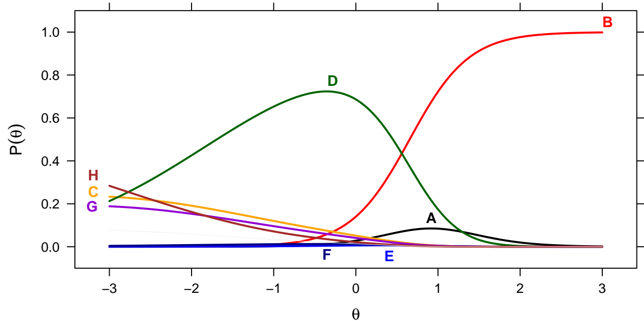
IRT Plot for Question 19
